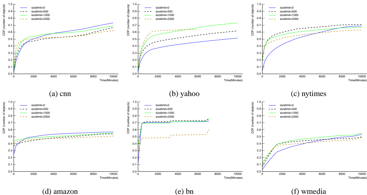
Fig. 2. The distribution of freshness time within different sizelimit for six dynamic web sites.
