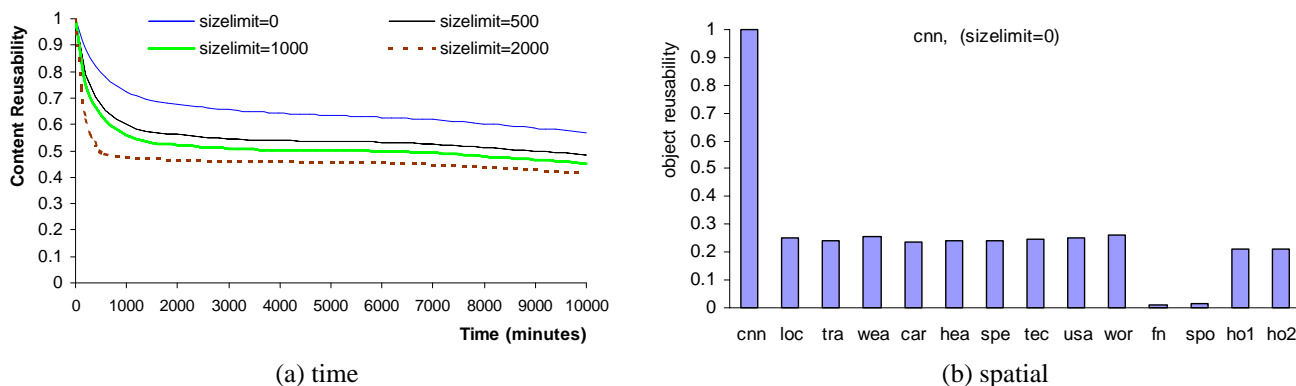
Fig. 3. Content reusability of cnn trace: (a) across time dimension, and (b) across linked documents.
