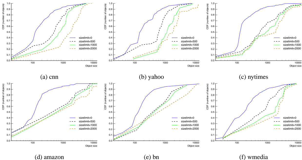
Fig. 1. The cumulative distribution function (of the number of objects) versus object size for different size limit settings for six dynamic web sites.
