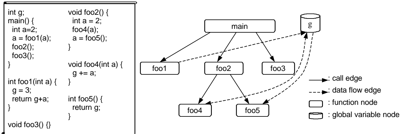
Figure 2. A sample program and its ASDG
