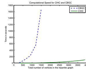
Figure 16: Computational speed comparison of CIHC with CBGC. The time required by each of the algorithms to compute the indicator vector are displayed for increasing number of vertices in the tripartite graph.
