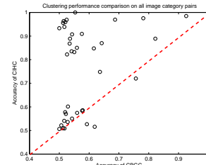
Figure 15: Clustering performance of CBGC and CIHC on all image category pairs. Each circle represents a possible category pair. Most of the circles fall in the upper part of the diagonal.
