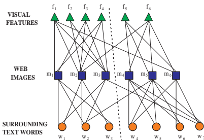
Figure 2: Tripartite graph of visual features, web images and the words coming from the surrounding text of the images.
