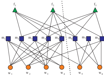
Figure 4: Toy problem of 3, 8 and 6 vertices of F , M and W , respectively with uniform weights along all edges. The dotted line shows the ideal cut for partitioning this graph.
